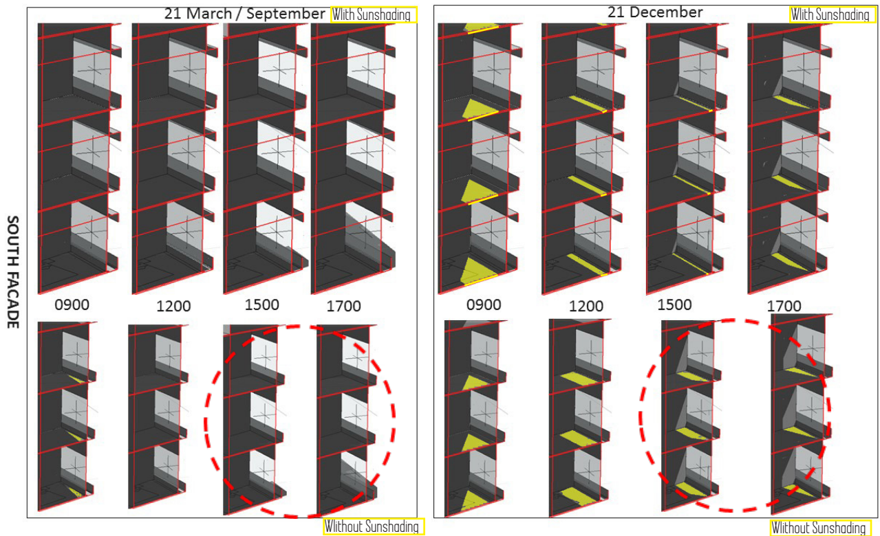
Figure 5.2.1.h Section of the room South façade
