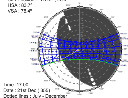
Figure. 5f: window NW,NE with sunshading
