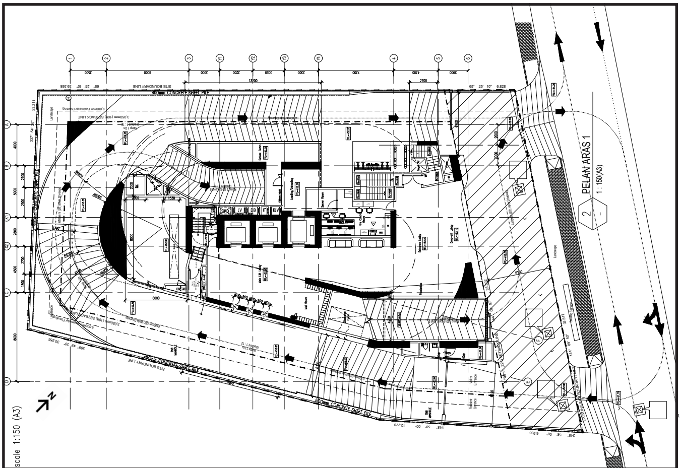
Figure 4: shows the level 2 of the building ( entrance )
