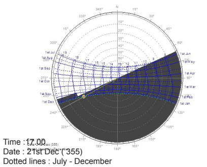
Figure 5c: window NW Windows without Sun Shading
