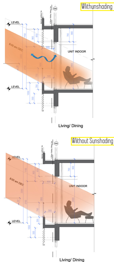
Section of the room NE façade
