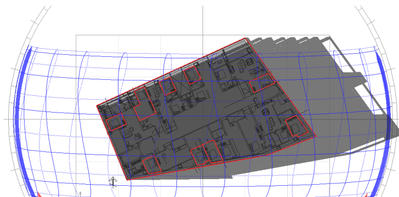
Figure 5.2 a Typical floor plan Solar penetration on 21 December
