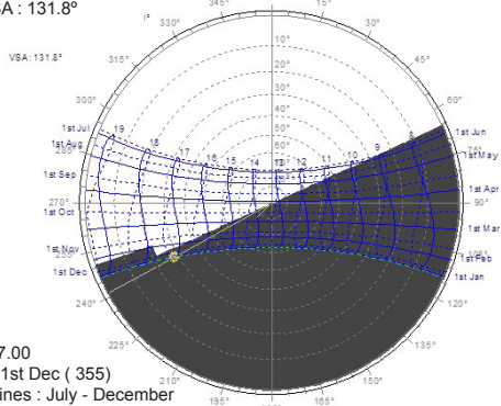
Figure. 5c: window NW Windows without Sun Shading
