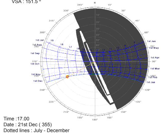
Figure 5b : Window SW without Sun Shading
