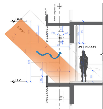
21 NW Sun Shading
