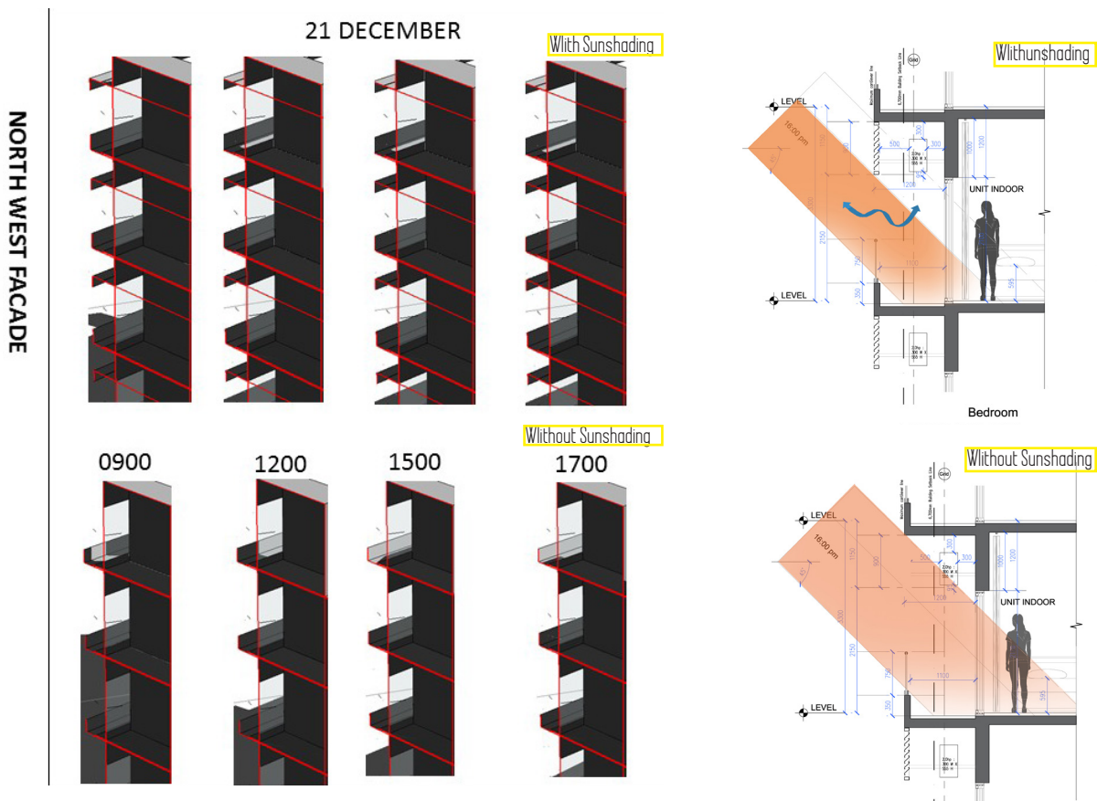
Figure 5.2.1.g Section of the room NW façade
