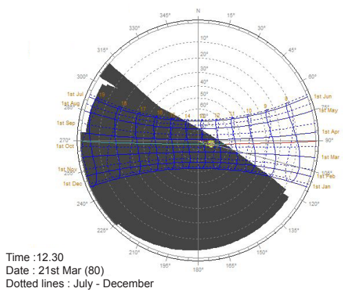
Figure 5a. Stereographic Diagram for windows at NE without Sun Shading (Solar Obstruction)
