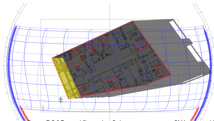
Figure 5.2 F Typical floor plan Solar penetration on 21 March and September
