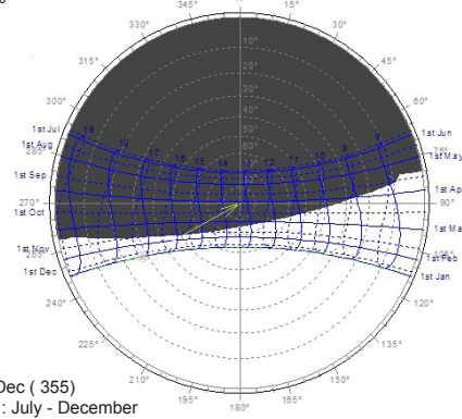
Figure. 5d : window S without Sun shading
