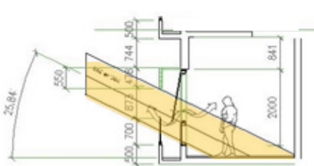
21 SOUTH EAST WITH SUN SHADING
