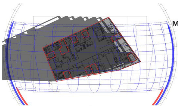
South Facade Solar Penetration Figure 5.4d (Page 22) Typical floor plan Solar penetration on 21 March and September at 9.00 am
