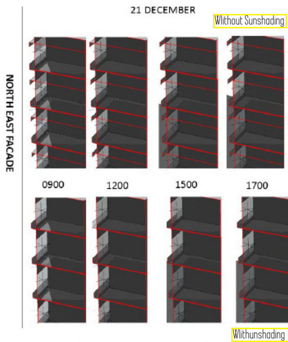
Figure 5.2.1.e Section of the room NE façade
