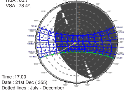
Figure 5f: window NW,NE with sunshading
