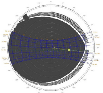
Figure 5e. sunning windows SW with sun shading
