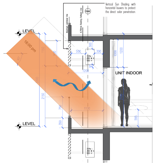
21 NW Sun Shading at 16.00pm
