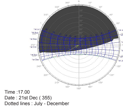
Figure 5d : window S without Sun shading
