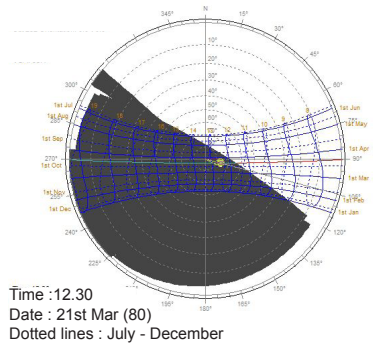
Figure 5a. Stereographic Diagram for windows at NE without Sun Shading
