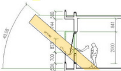
21 SOUTH WEST WITH SUN SHADING
