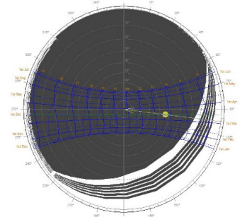
Figure 5g: window SE and NE Windows with Sun Shading
