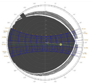
Figure . 5e. sunning windows SW (solar obstruction)
