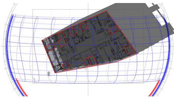
South Facade Solar Penetration Figure 5.3.c (Page 21) Typical floor plan and solar penetration on 21 December at 17.00 pm
